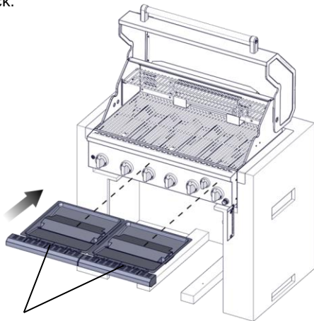
Grease Tray
