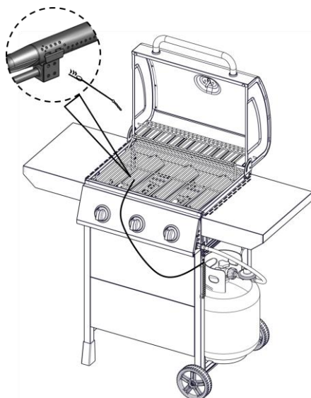
Main burner
