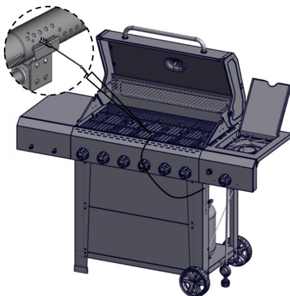
Main burner
