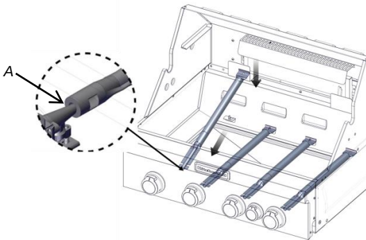
A. Burner/orifice connection
