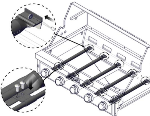
A. Burner/orifice connection
