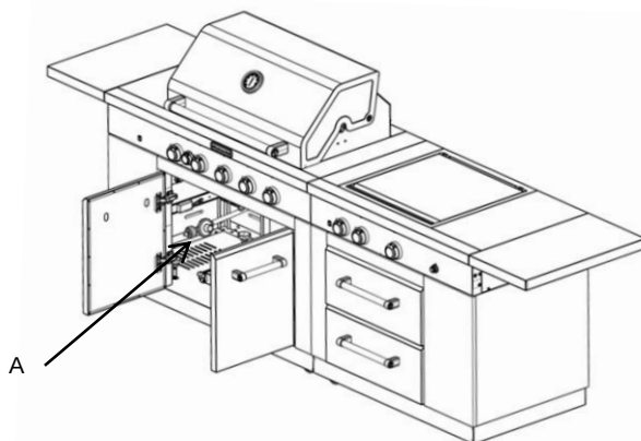
A. Gas pressure regulator/hose assembly
