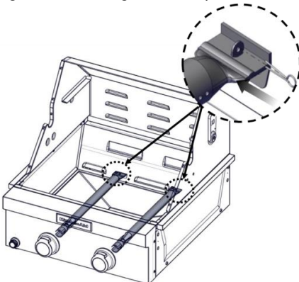
A. Burner/orifice connection
