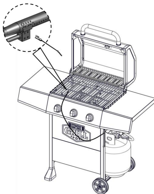
Main burner
